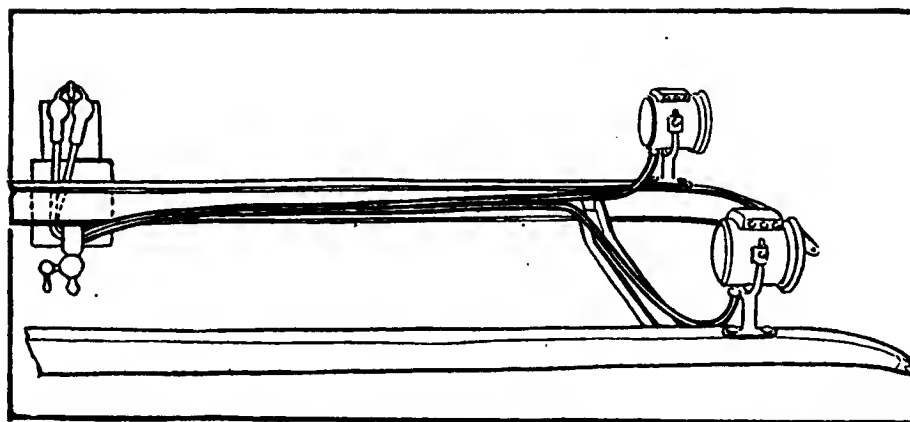
Fig. 3—How a trap may be interposed in the acetylene gas lead in order to catch water and mechanical impurities
